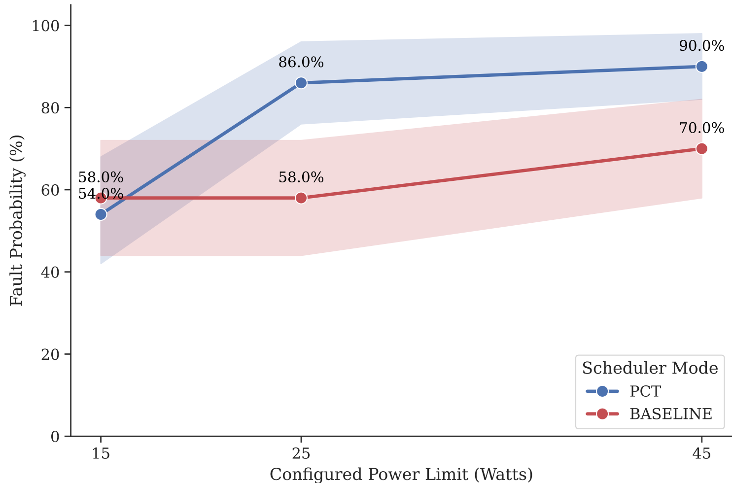
Figure 1: Concurrency Fault Manifestation Rate Across Thermal-Power Constraints
